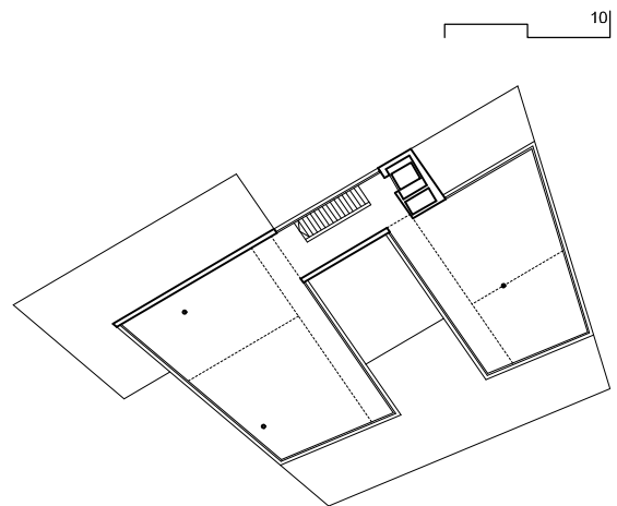
Attikageschoss
